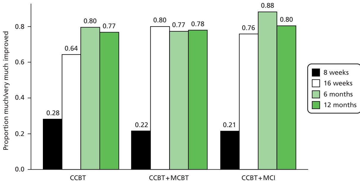
FIGURE 4 Child CGI-I.
