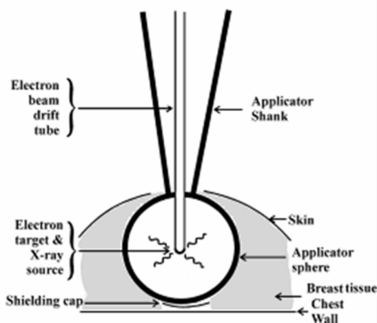
Figure 2: The Intrabeam System (PRS). The electrons are generated and accelerated in the main unit and travel via the electron beam drift tube which is surrounded by the conical applicator sheath such that its tip lies at the epicentre of the applicator sphere. Once the electrons hit the inner surface of the hemisphere at the tip, x-rays are generated. Thus a uniform radiation dose rate is available at the surface of the applicator sphere 8 . The details of operative technique are available at http://www.targit.org.uk .
