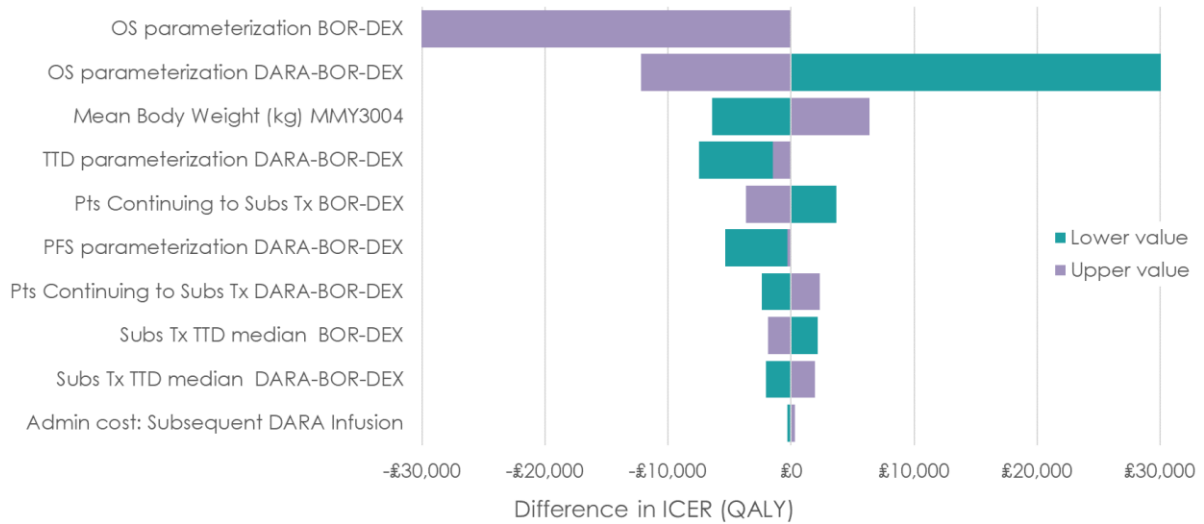
Figure 13 Tornado plot DBd vs Bd: ERG corrected company base case (list prices)
