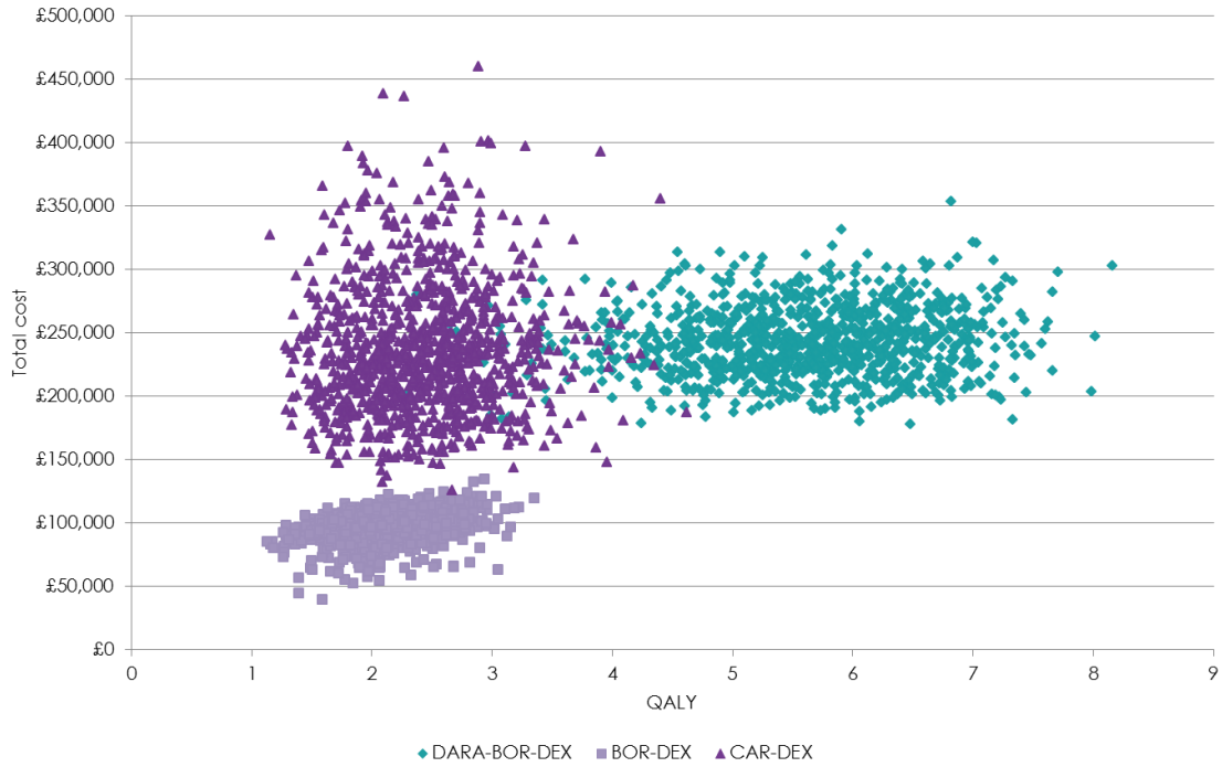
Figure 15 Scatter plots for ERG corrected company base case (list prices)
