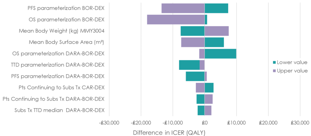
Figure 14 Tornado plot DBd vs Cd: ERG corrected company base case (list prices)
