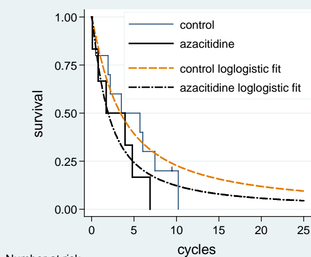
Survival in AML; SDC subgroup
