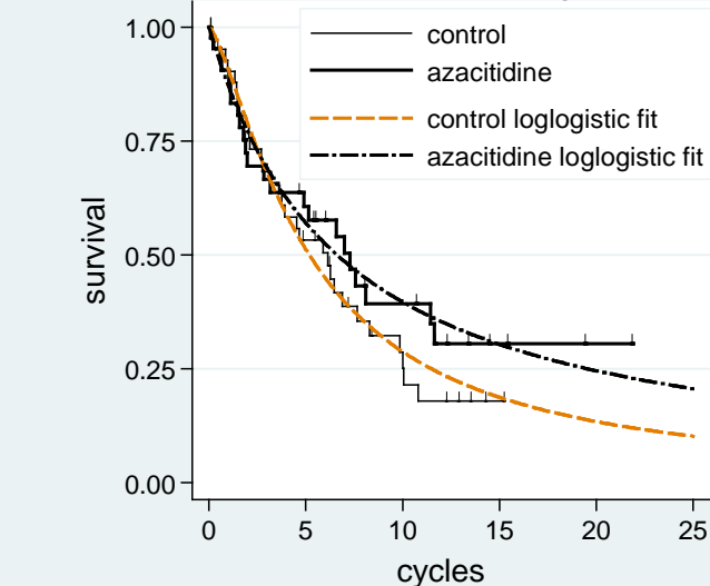
Survival in AML; BSC subgroup
