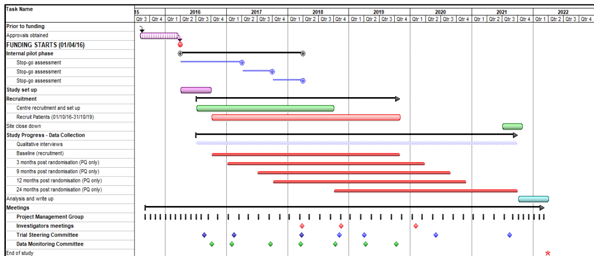
Figure 3: Gantt Chart
