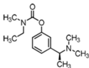
Figure 4: Structure Rivastigmine
