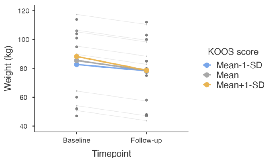
Figure 4. Subgroup analysis example: KOOS scores and weight change over time (mock data).
