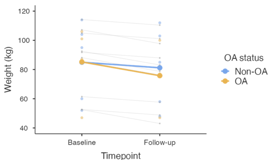
Figure 3. Main analysis example: OA status and weight change over time (mock data).
